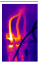
Contactor
